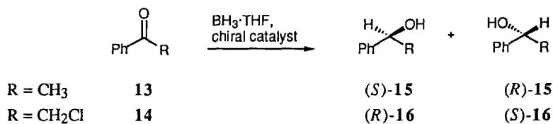
Scheme 1: Enantioselective catalytic reductions of prochiral ketones with the oxazaphospholidine oxides 4-10 and excess borane in THF 12
